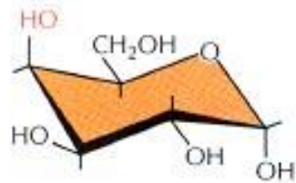
\alpha -D-Galactose (Gal)
