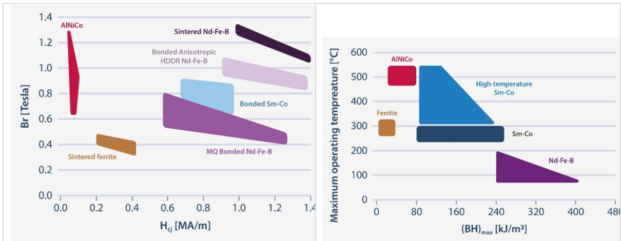
Figure 387: (left) Comparison of the properties of different types of magnets. Br = remanence (magnetization left after an external magnetic field is removed); H cj = coercivity (a measure of the resistance of a ferromagnetic material to becoming demagnetized) (Binnemans 2018). (right) Comparison of the maximum operating temperatures of NdFeB and Sm-Co magnets (Binnemans 2018).
