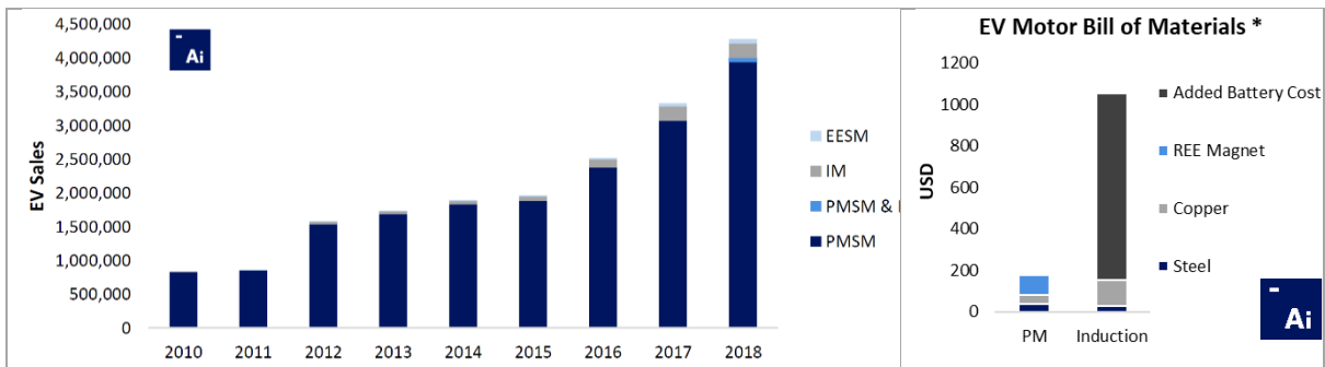
Figure 324: Left: Over 90% of all EVs produced to-date have used permanent magnet traction motors (PMSM). IM - induction motors, EESM - electrically-excited synchronous motors. Right: Added battery pack costs incurred by an automaker using less efficient motor type (Adamas Intelligence 2019)
