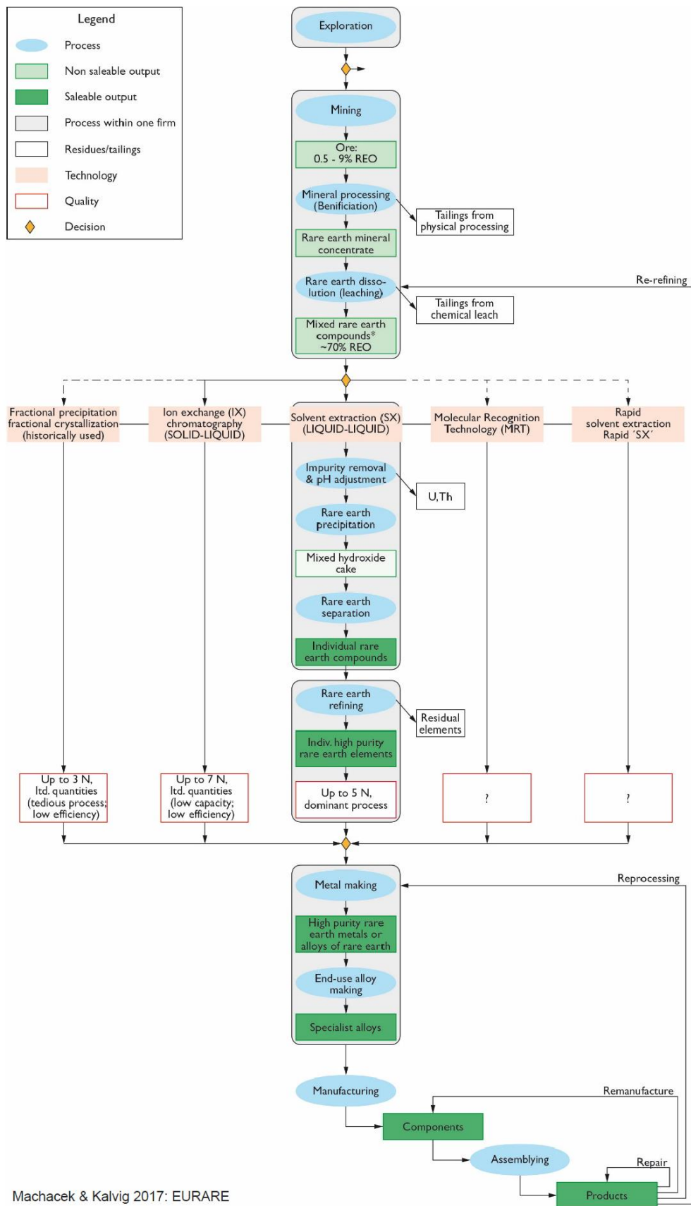
Figure 409: Generic material supply chain for REE. Source: MiMa-GEUS, 2016 based on Gupta and Krishnamurty, 2005 (Machacek and Kalvig 2017: EURARE)
