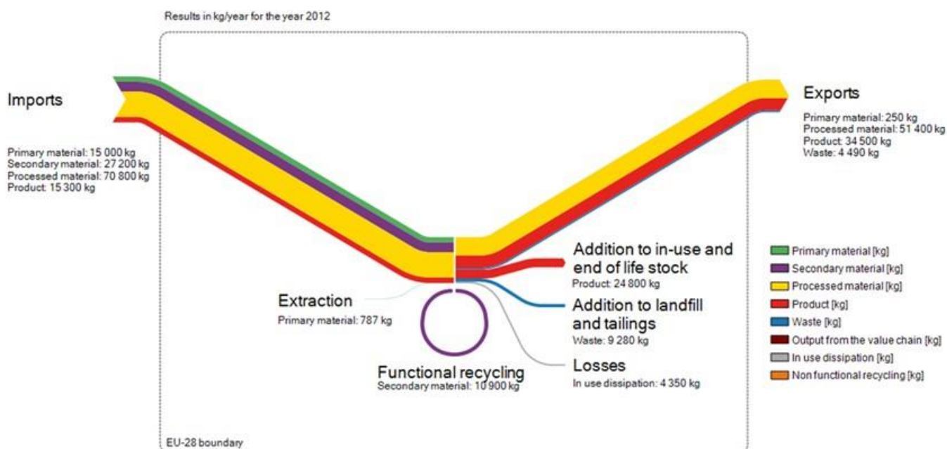
Figure 291: Simplified MSA of palladium flows in the EU for 2012. (BIO Intelligence Service, 2015a)
