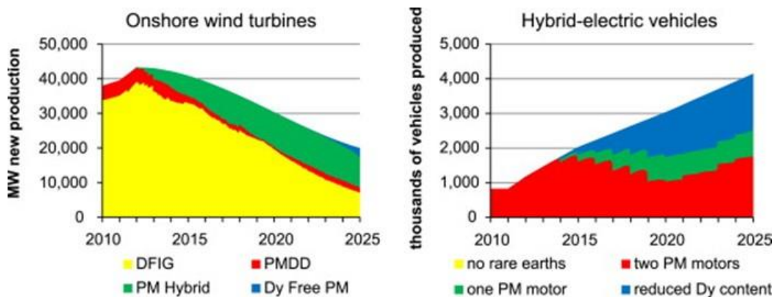
Figure 394: Production of onshore wind turbines and hybrid electric vehicles using different technologies: average baseline scenario projections. (Notes:
