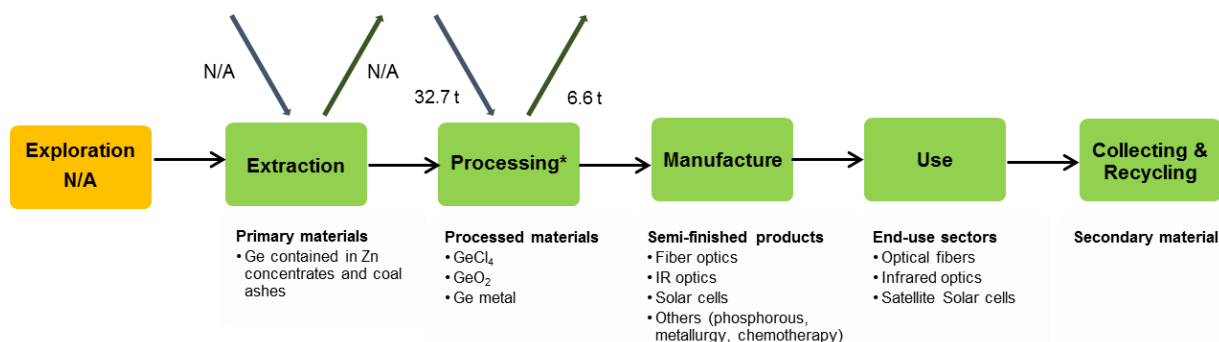
Figure 139: Simplified value chain for germanium 99 for the EU, averaged over 2012-2016
