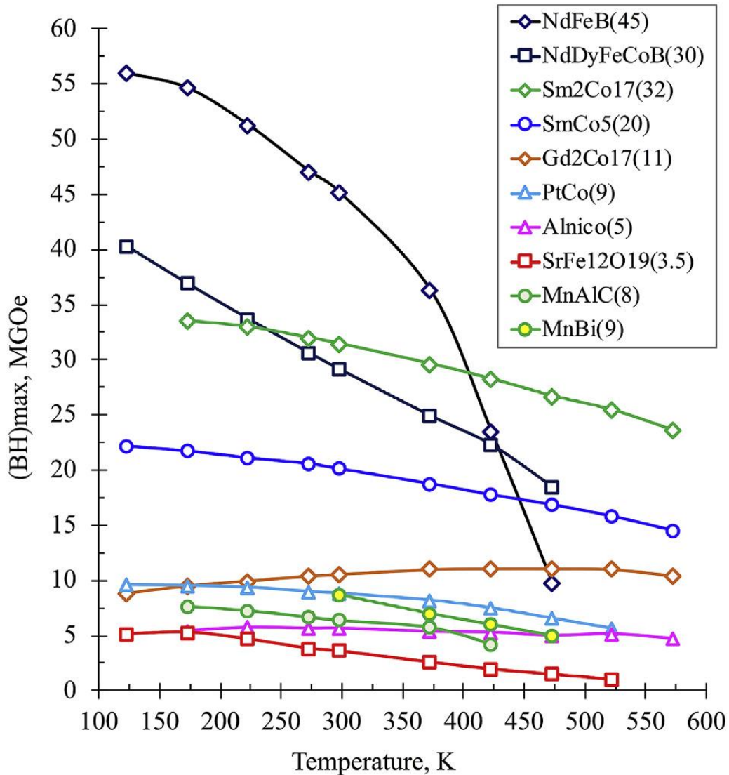
Figure 407: Magnets strength (BH)_{max} of most commercial permanent magnets changing with temperature. The value in parentheses in (BH)_{max} at 298 K (25°C). (Cui et al. 2018)
