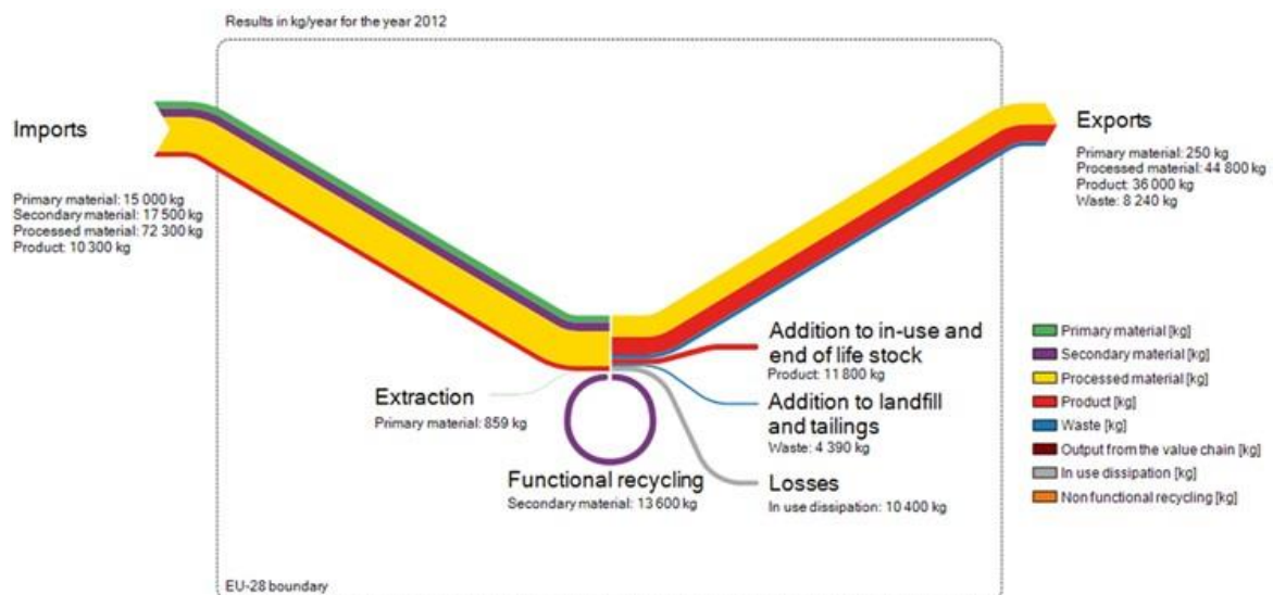
Figure 292: Simplified MSA of platinum flows in the EU for 2012. (BIO Intelligence Service, 2015a)
