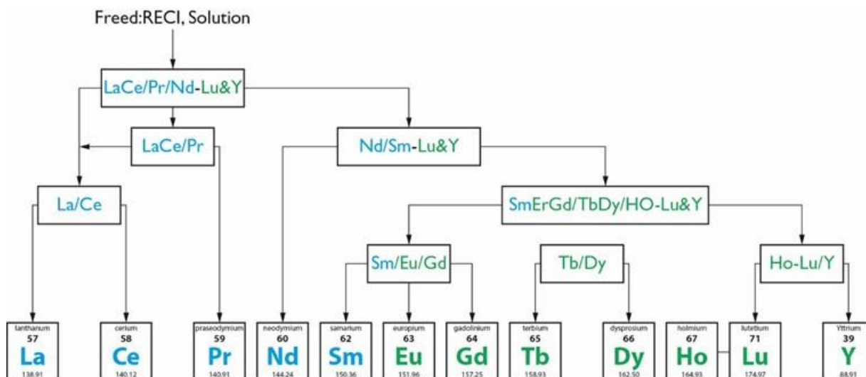
Figure 445: Example of a schematic REE solvent extraction (SX) separation process (Machacek and Kalvig 2017: EURARE adapted from Zhang and Zhao, 2016)
