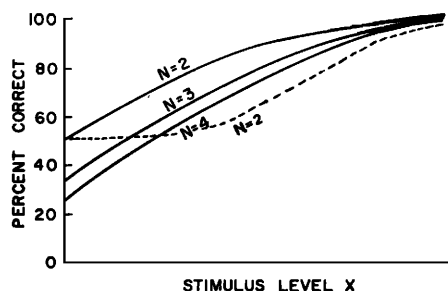
FIG. 2. The solid curves show the expected proportion of correct responses, assuming the stimulus level is directly proportional to d' . The parameter N is the number of alternatives. The dashed curve shows a psychometric function derived from the normal ogive in which an adjustment for chance responses has been made.
