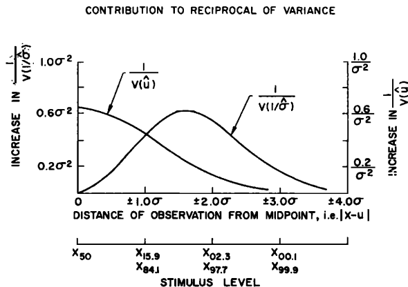
FIG. 3. Contribution to reciprocal of error variance. The two curves show the expected increase, with each new observation, in the reciprocal of the error variance for the estimates of 1/\sigma and \mu , respectively. The predictions are for the large-sample maximum-likelihood estimates assuming a cumulative normal response curve. Ideally, the observations should be symmetrically placed about \mu .
