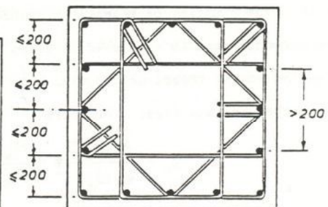
Four overlapping hoops
