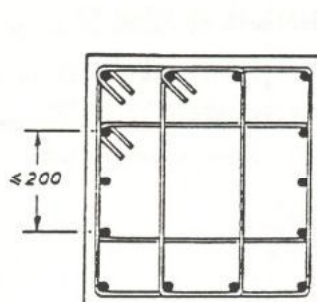
Three overlapping hoops
