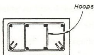
Two overlapping hoops - not preferred
