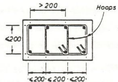
Two overlapping hoops - preferred detail
