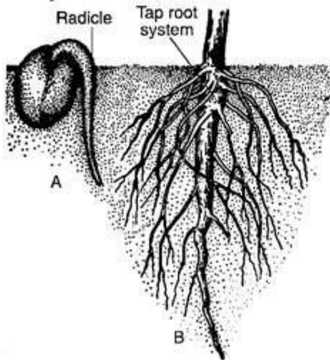
Fig. 2.19 : Tap root system in dicotyledonous plants : A. Germinating seed, B. Tap root system
