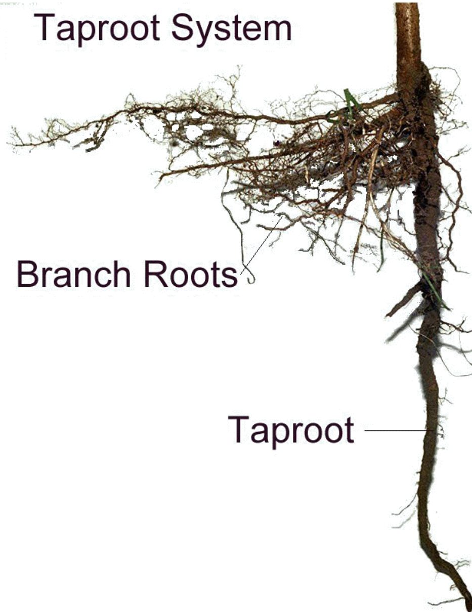
Fig. 2.19 : Tap root system in dicotyledonous plants : A. Germinating seed, B. Tap root system
