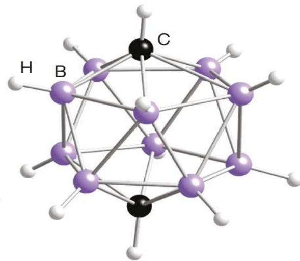
closo -1,12- \text{B}_{10}\text{C}_2\text{H}_{12}
