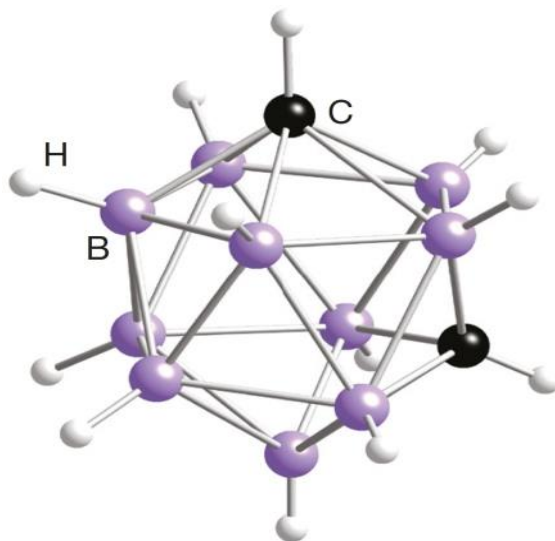
closo -1,7- \text{B}_{10}\text{C}_2\text{H}_{12}
