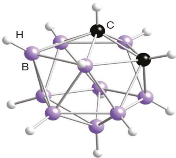
closo -1,2- \text{B}_{10}\text{C}_2\text{H}_{12}
