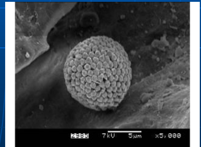
Pirite framboidale
