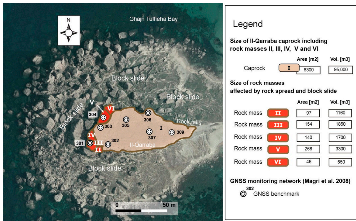
Figure 6. Map showing the location of Il-Qarraba caprock and its rock masses displaced by rock spreading and block sliding. Tilted megablocks transported by block slides are clearly visible (background GE image).
