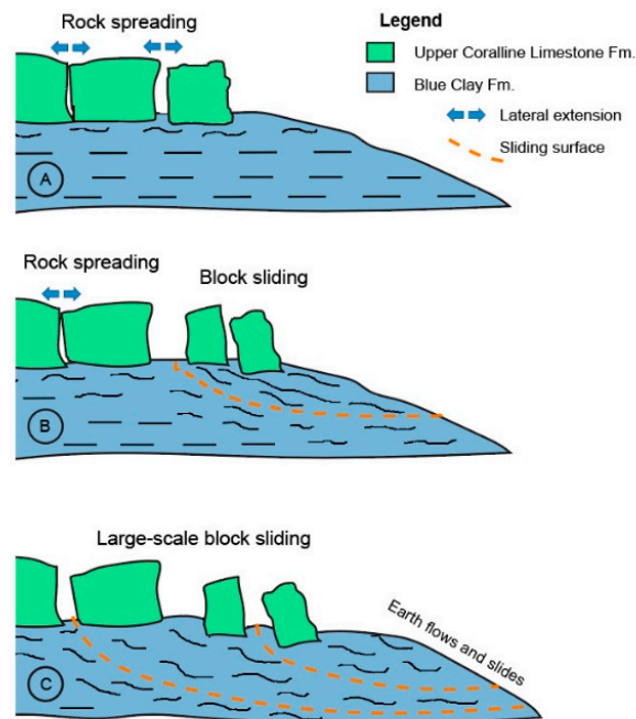
Figure 3. Landslide evolution along the northwestern coast of Malta. Schematic and simplified examples of (A) early stage of rock spreading; (B) lateral spreading evolving into block sliding; and (C) advanced stage of landsliding (cf. [52]).
