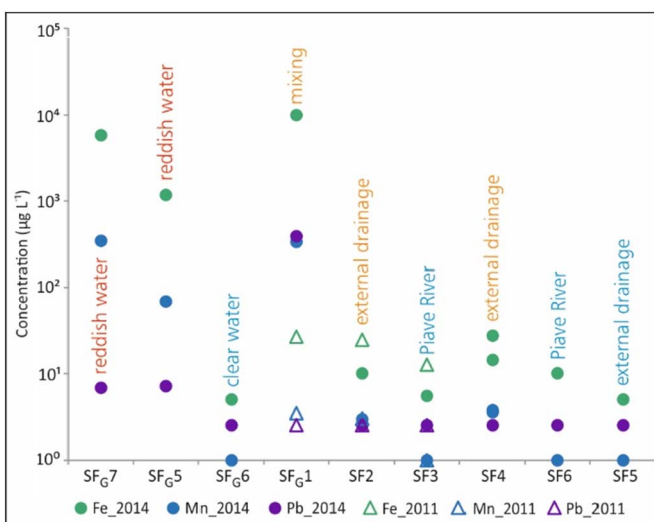
Fig. 5. Effect of dilution process observed for Pb, Fe and Mn in the drainage waters flowing from the inner part of the mine towards the Piave River.
