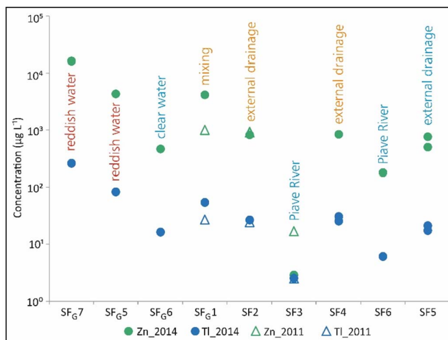
Fig. 4. Effect of dilution process observed for Zn and Tl in the drainage waters flowing from the inner part of the mine towards the Piave River.
