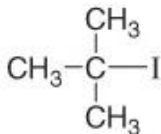
Ter-butyl ioduro
