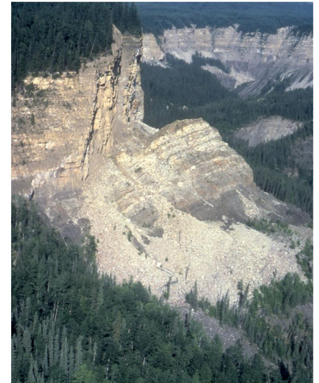
Fig. 6 A rotational slide involving Cretaceous shale, overlain by sandstone. Liard Plateau, Canada (Photo by O. Hungr)
