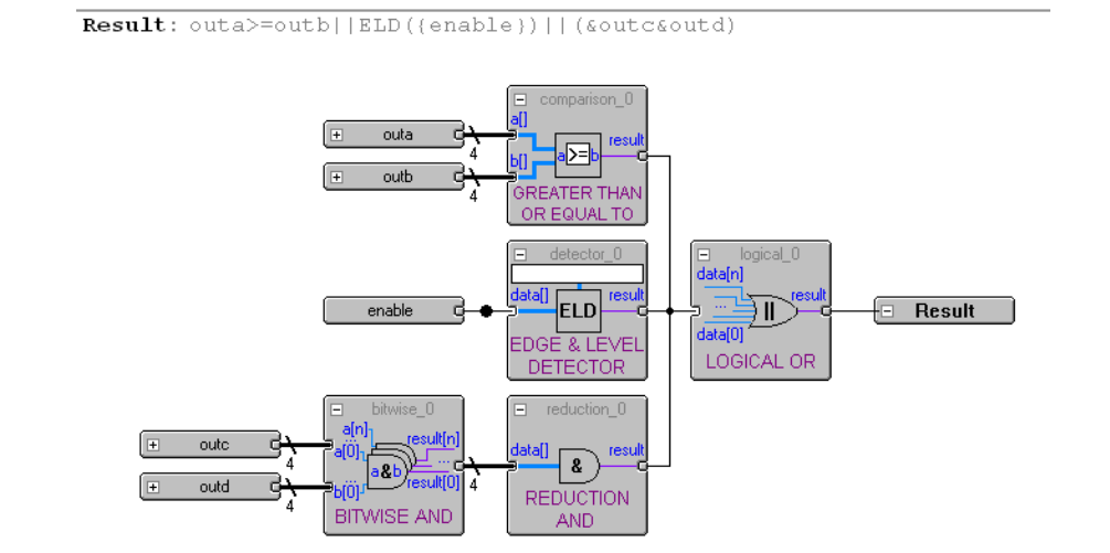
Figure 13-23. Bitwise AND Operation
