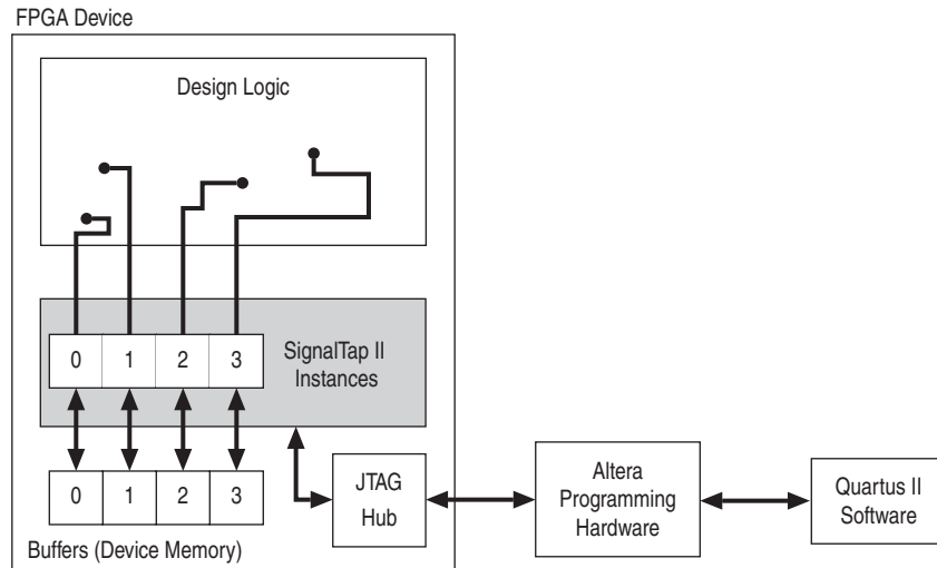
Figure 13-1. SignalTap II Logic Analyzer Block Diagram (1)
