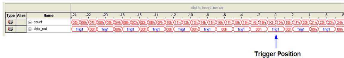
Figure 13-39. SignalTap II Logic Analyzer Continuous Data Capture (1)
