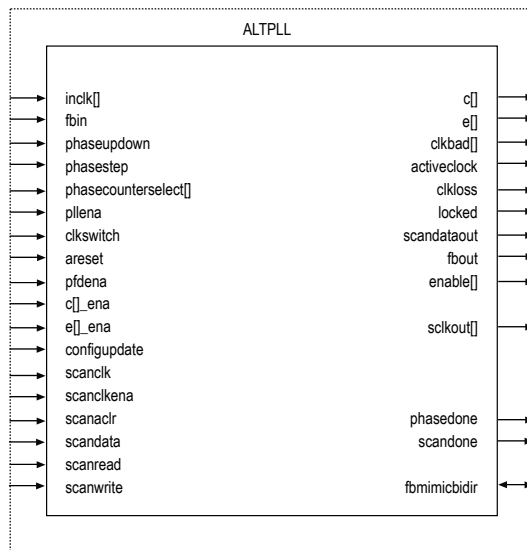
Figure 24: Input and Output Ports of the ALTPLL Megafunction Block
