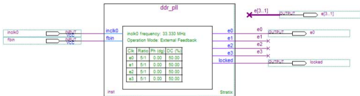
Figure 20: ALTPLL ddr_pll Design Schematic
