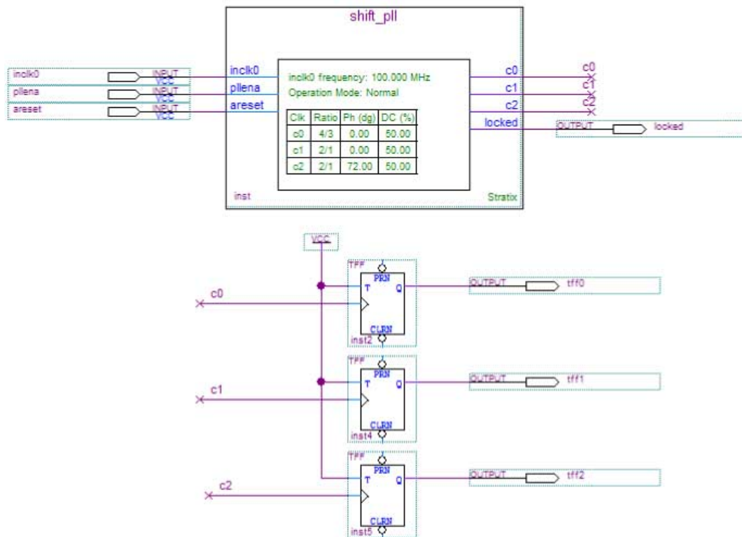
Figure 22: ALTPLL shift_pll Design Schematic
