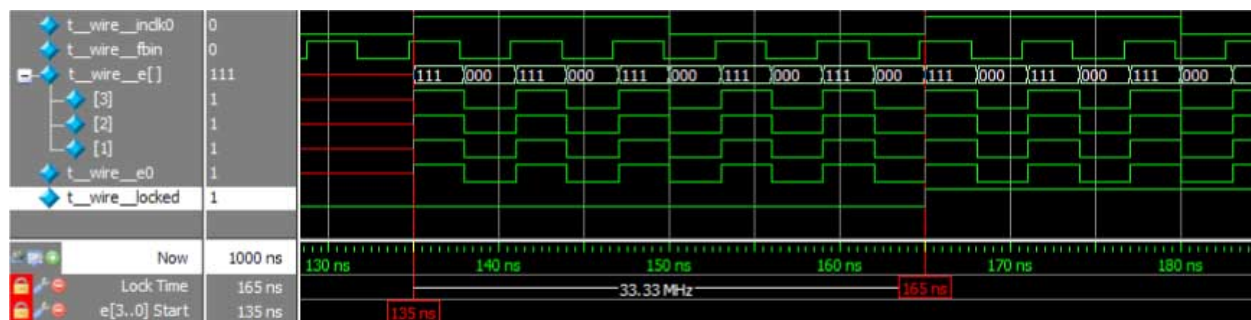
Figure 21: ModelSim Simulation Results
