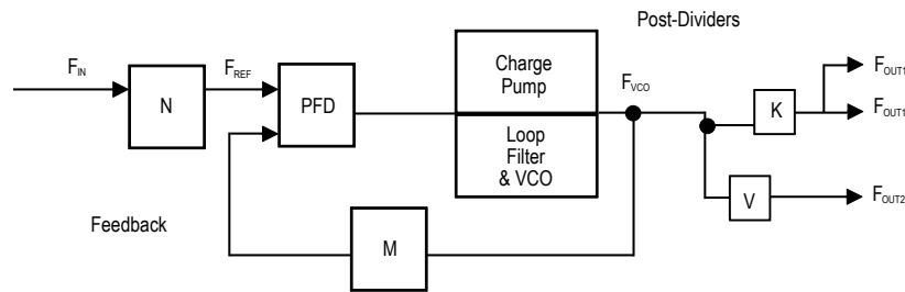
Figure 1: PLL Block Diagram
