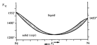
FIGURE 6-52. Positive deviation from ideality in the Pd-Ni solid solution system. (From Hansen.) Compare Figure 6-40.
