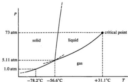
FIGURE 5-9. The PT phase diagram for carbon dioxide. Dry ice sublimates at normal pressures because this pressure is less than that of the triple point for CO 2 . At pressures above 5.11 atm dry ice will melt in what we usually think of as a “normal” manner.
