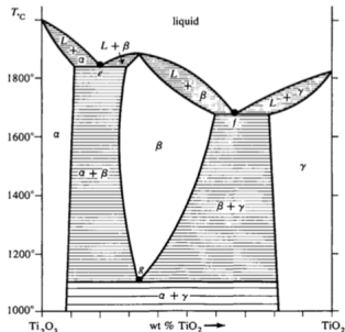
FIGURE 6-61. The \text{Ti}_2\text{O}_3 - \text{TiO}_2 portion of the full Ti-O phase diagram, showing two eutectic points e and f and a eutectic point g. This diagram can be thought of as the next logical step in the sequence begun in Figure 6-60.
