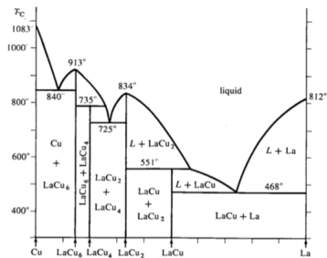
FIGURE 6-64. A compound phase diagram of Cu, La, and four intermediate compounds, all mutually insoluble in the solid phase. This diagram can be considered as being built up from simple diagrams such as Figures 6-58 and 6-63.
