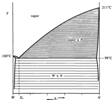
FIGURE 6-48. Phase diagram at 1 atm pressure for water (W) and nitrobenzene (N), to illustrate the process of steam distillation.
