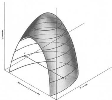
FIGURE 6-26. The complete pressure-temperature-composition diagram for two partially miscible liquids. Figures 6-22 to 6-25 are sections normal to the P axis. The ends of the tie line ab give the compositions of the two immiscible phases which will be present for any P , T , and X_1 point falling on the tie line. The relative molar amounts of the two phases will be given by the position of the PTX point on the tie line, in accordance with the lever principle. ( X_1 is the over-all composition of both phases.)
