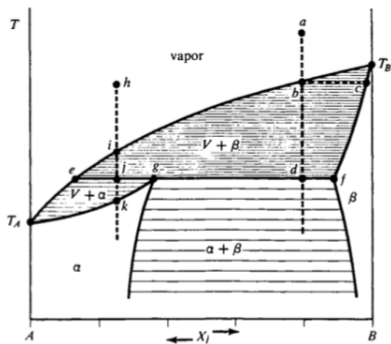
FIGURE 6-47. The liquid-vapor analog of peritectic behavior in solid-liquid systems (Figure 6-57).
