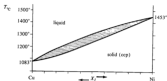
FIGURE 6-51. Melting point diagram for the Cu—Ni system, which shows nearly ideal solid solution behavior. The lower curve is the solid composition and the upper curve is the liquid composition in equilibrium with it at a given temperature. The interpretation, including the use of the lever principle, is identical to that of Figure 6-30. [From M. Hansen, The Constitution of Binary Alloys (McGraw-Hill, New York, 1958).]
