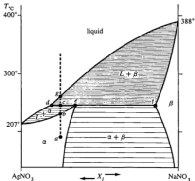
FIGURE 6-57. Peritectic behavior in a system with a range of compositions possible in the solid phases.
