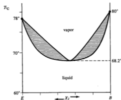
FIGURE 6-40. Boiling point diagram at 1 atm for the ethanol-benzene system, showing a minimum-boiling azeotrope. Fractionation of a solution to the left of the azeotropic composition would yield pure ethanol and a distillate of the constant azeotropic composition. From this figure and Figure 6-39, try to imagine the full PTX diagram for positive deviation, analogous to Figures 6-33 and 6-38.
