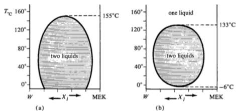
FIGURE 6-25. Miscibility of methyl ethyl ketone (MEK) and water (W) at moderate pressures (a) and at 150 atm pressure (b). The vapor pressure of water at the upper consolute temperature of 155°C is approximately 5 atm, and the vapor pressure becomes 150 atm at 343°C.
