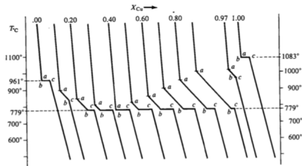
FIGURE 6-56. A family of cooling curves for the Ag-Cu system of Figure 6-55. The region from the top of the curve to point a represents cooling of the liquid. From a to b , the liquid is continuing to cool, but at a slower rate since a solid phase is crystallizing out and giving off its heat of fusion. Section b to c is a eutectic halt until the last liquid crystallizes, longer or shorter depending on how much liquid was left when the liquid composition reached the eutectic point ( w in Figure 6-55). From c to the bottom of the diagram, the solid phase or phases are cooling. It is from information such as these curves provide that phase diagrams like Figure 6-55 are constructed.
