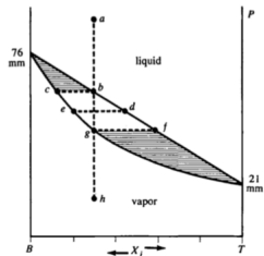
FIGURE 6-29. Composition of liquid and vapor as a function of pressure at 20°C for benzene (B) and toluene (T), which form a nearly ideal solution. The straight liquid-composition line has been seen before in Figure 6-1, but at 25°C.
