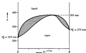
FIGURE 6-39. Vapor pressure diagram of a solution of ethanol (E) and benzene (B), showing positive deviation. The upper, liquid composition curve is analogous to the acetone-carbon disulfide curve of Figure 6-13.
