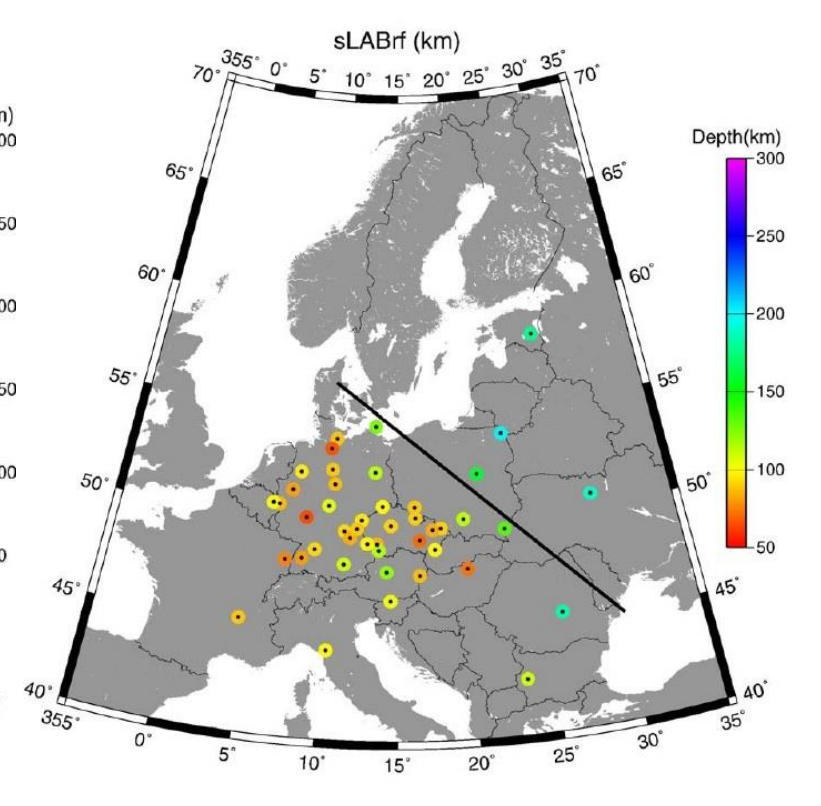
Seismic LAB (receiver functions)
