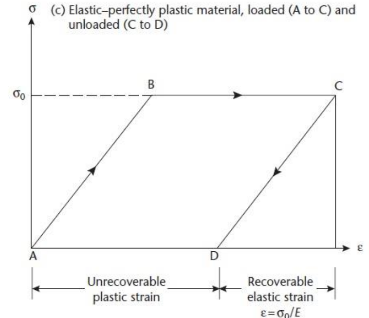
Relationship between stress \sigma and strain \epsilon for elastic and ductile deformation
