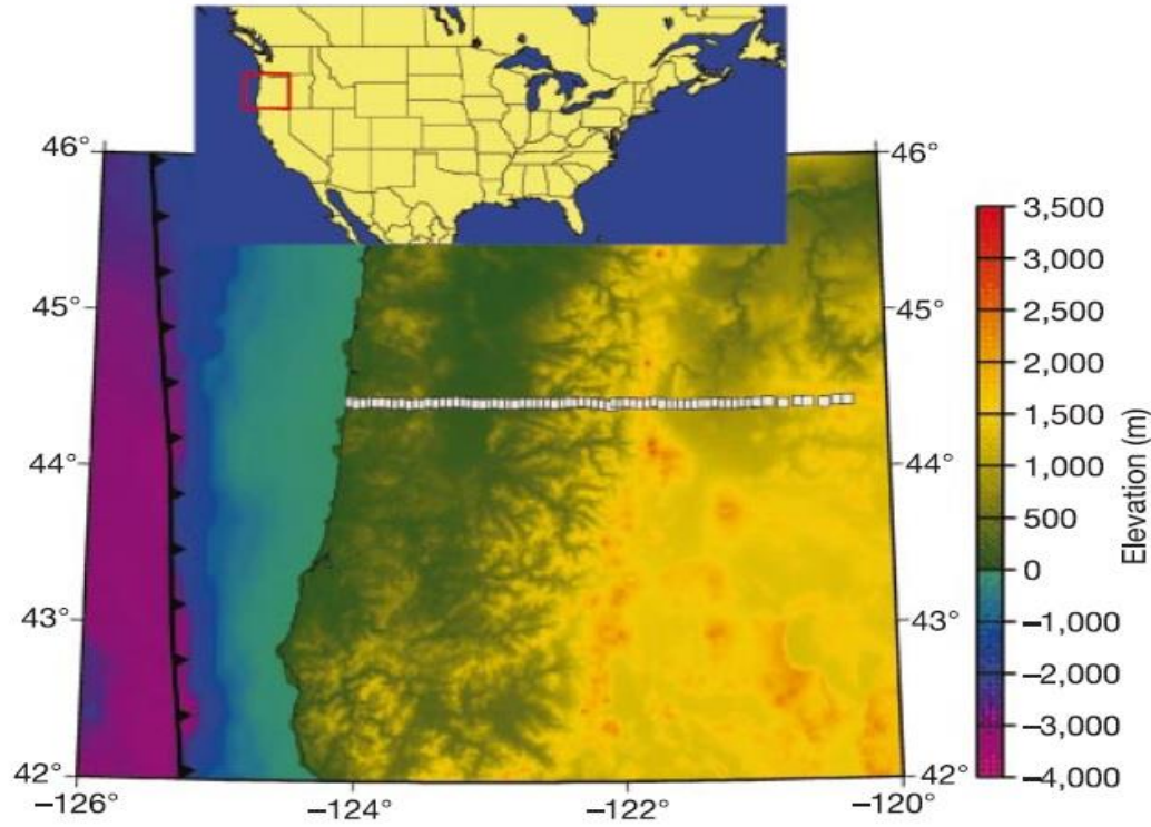
Bostock et al., 2002, Nature, 417
