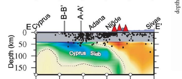
Govers and Fichtner, 2016, EPSL, 450
