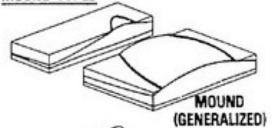
MOUND TYPES
