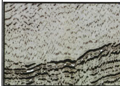
Facies Change
