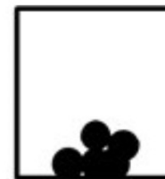
Sedimentation
