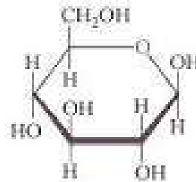
GLUCOSIO
