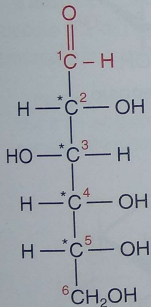
D-glucosio
