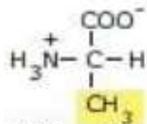
Alanina
