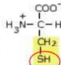
Cisteina
