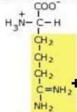
Arginina
