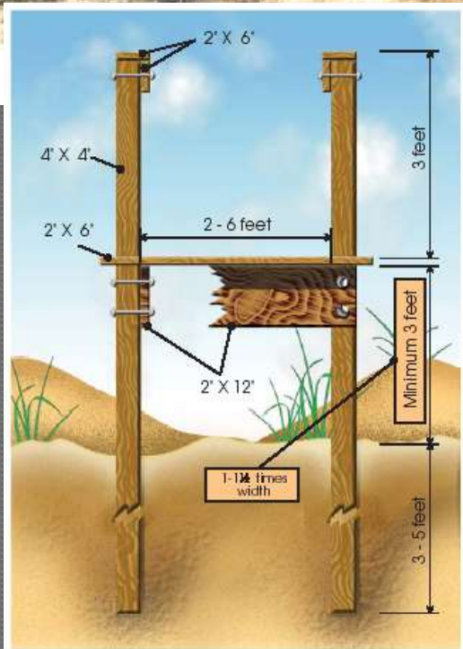
Figure 24. Construction details for a dune walkover.
