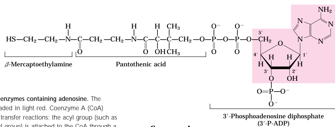
Coenzyme A
