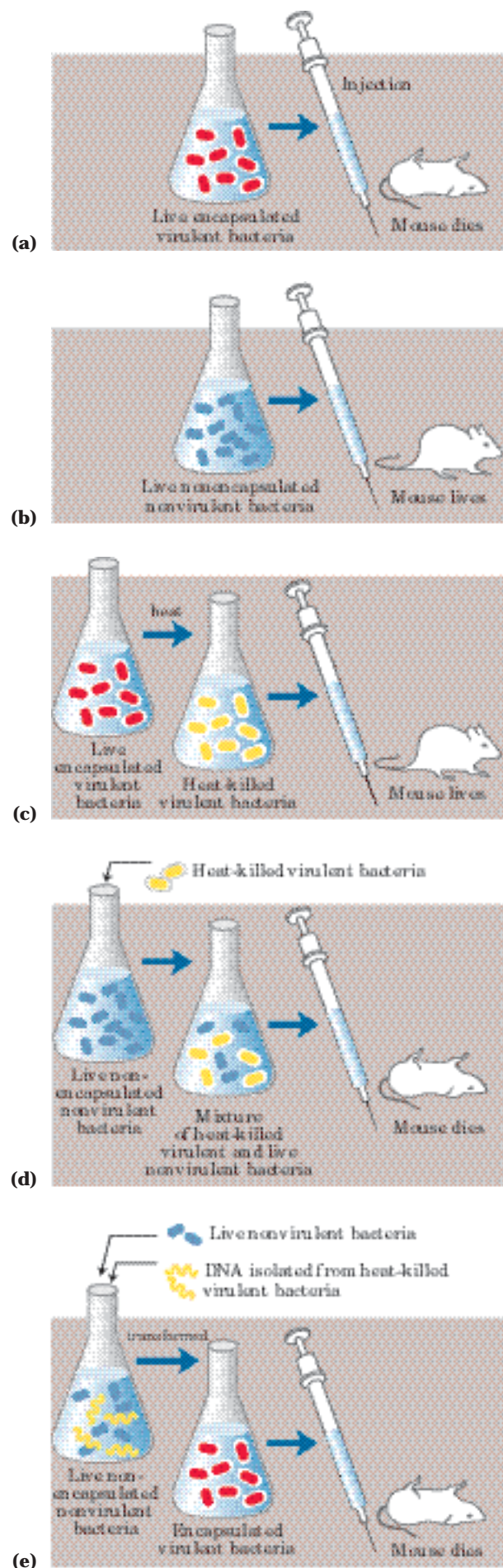
FIGURE 8-12 The Avery-MacLeod-McCarty experiment. (a) When injected into mice, the encapsulated strain of pneumococcus is lethal, (b) whereas the nonencapsulated strain, (c) like the heat-killed encapsulated strain, is harmless. (d) Earlier research by the bacteriologist Frederick Griffith had shown that adding heat-killed virulent bacteria (harmless to mice) to a live nonvirulent strain permanently transformed the latter into lethal, virulent, encapsulated bacteria. (e) Avery and his colleagues extracted the DNA from heat-killed virulent pneumococci, removing the protein as completely as possible, and added this DNA to nonvirulent bacteria. The DNA gained entrance into the nonvirulent bacteria, which were permanently transformed into a virulent strain.
