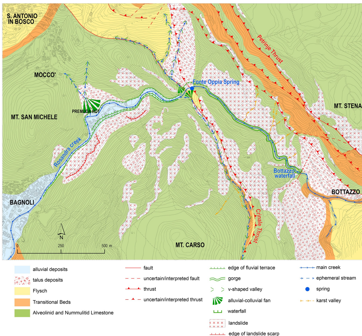
Fig. 4 - Geological map with geomorphological elements of the Rosandra creek and surroundings. The geological map is redrawn from Cucchi et al. (2013) and Jurkovšek et al. (2016).
