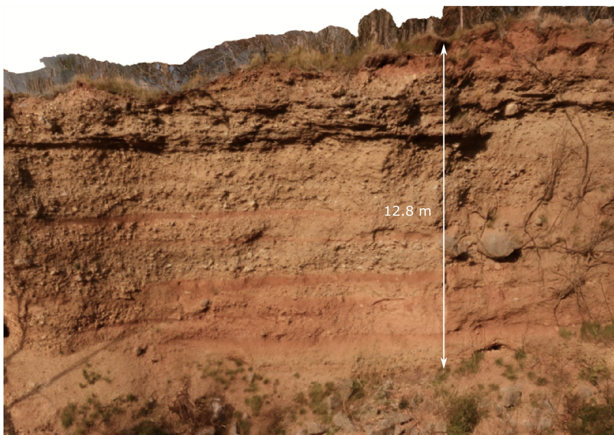
Fig. 6 - The stratigraphic sequence cropping out along the scarp of the terrace in front of the Premuda Hut (Bagnoli, Trieste).
