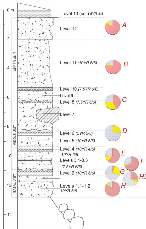
Fig. 7 - Stratigraphic description of the Premuda sequence. The circle diagrams show the percentage of gravel (red), sand (yellow) and mud (blue).
