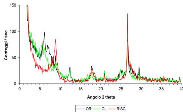
Fig. 9 - XRD of clay fraction on oriented, glycolated and heated glass slides.
