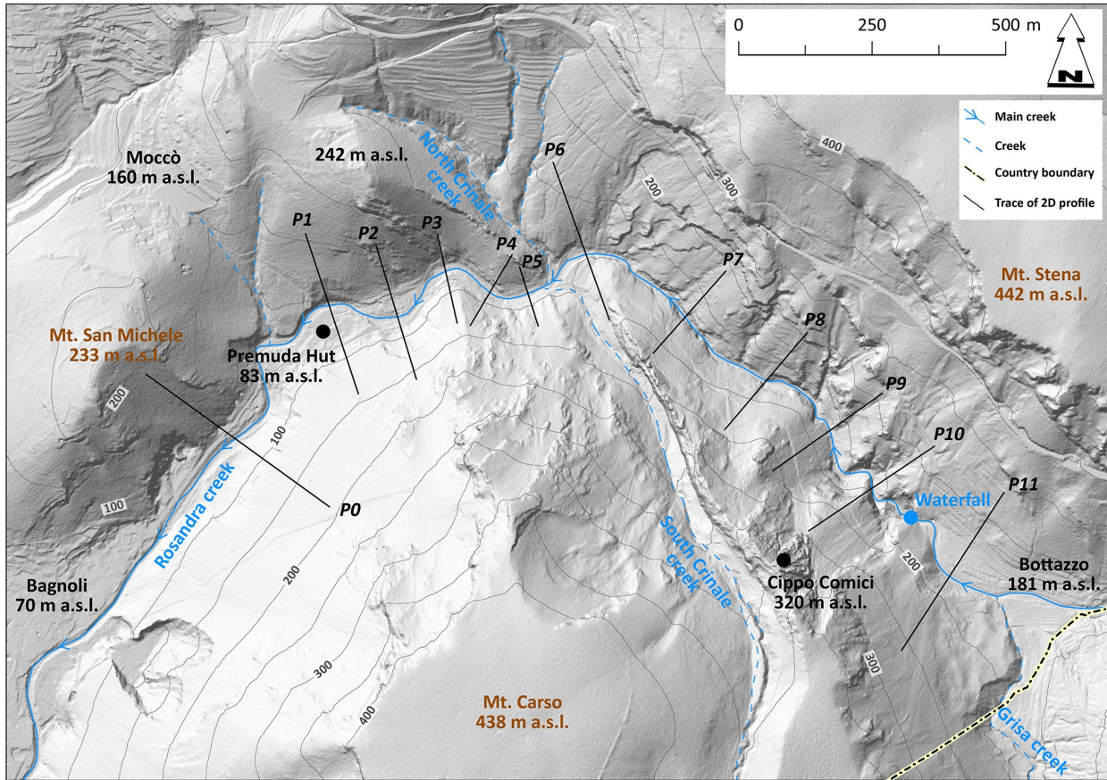
Fig. 2 - Hillshade of the study area realized through the processing of LiDAR data from Friuli Venezia Giulia Region. The profiles across the Rosandra Valley are numbered from 0 to 11.
