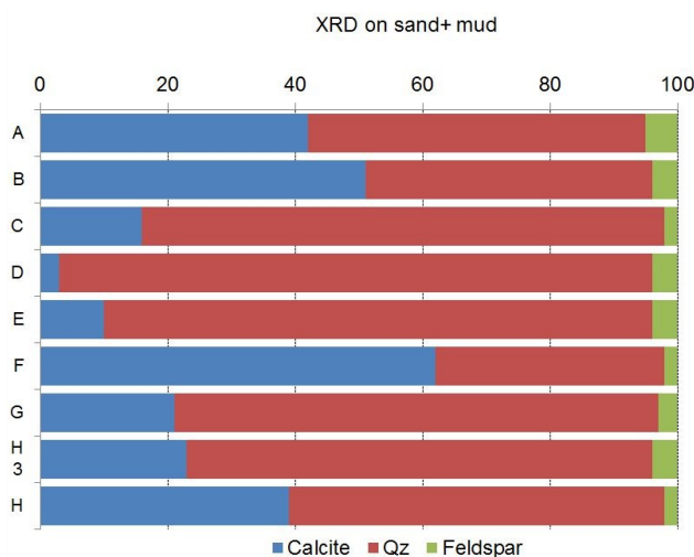
Fig. 8 - Percentages of calcite, quartz and feldspars in the studied layers by means of XRD.
