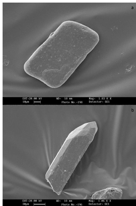
Fig. 10 - a) aluminum silicate in layer E; b) zircon in layer C.
