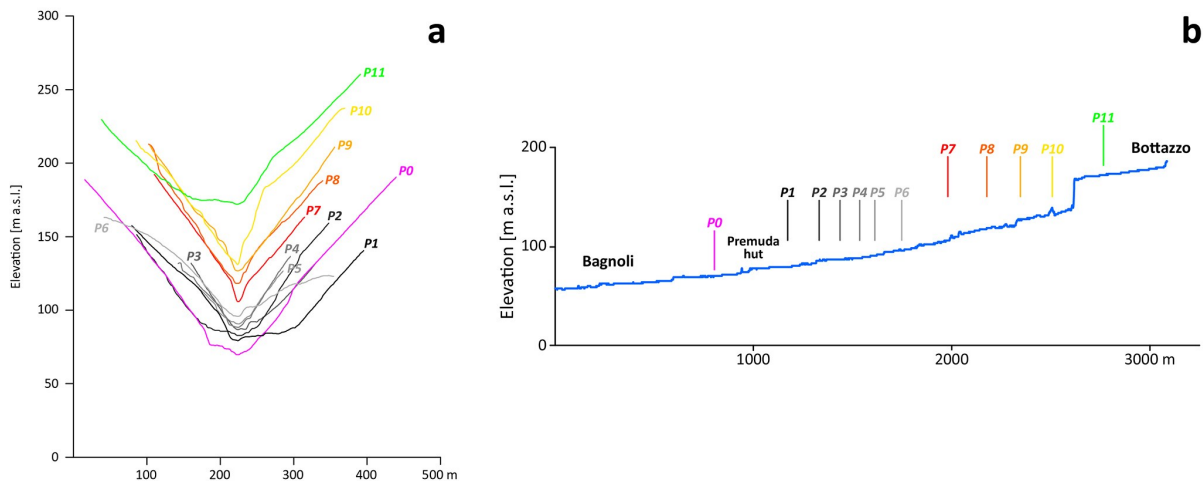
Fig. 3 - The profiles along the Rosandra creek: a) the overlapping of the profiles shows the uppermost one (green), near Bottazzo, 4 profiles in the gorge (yellow to red), and 6 profiles in the lower part of the creek (grey shades). The Profile 0 is out of the study area (magenta); b) longitudinal profile of the Rosandra creek.
