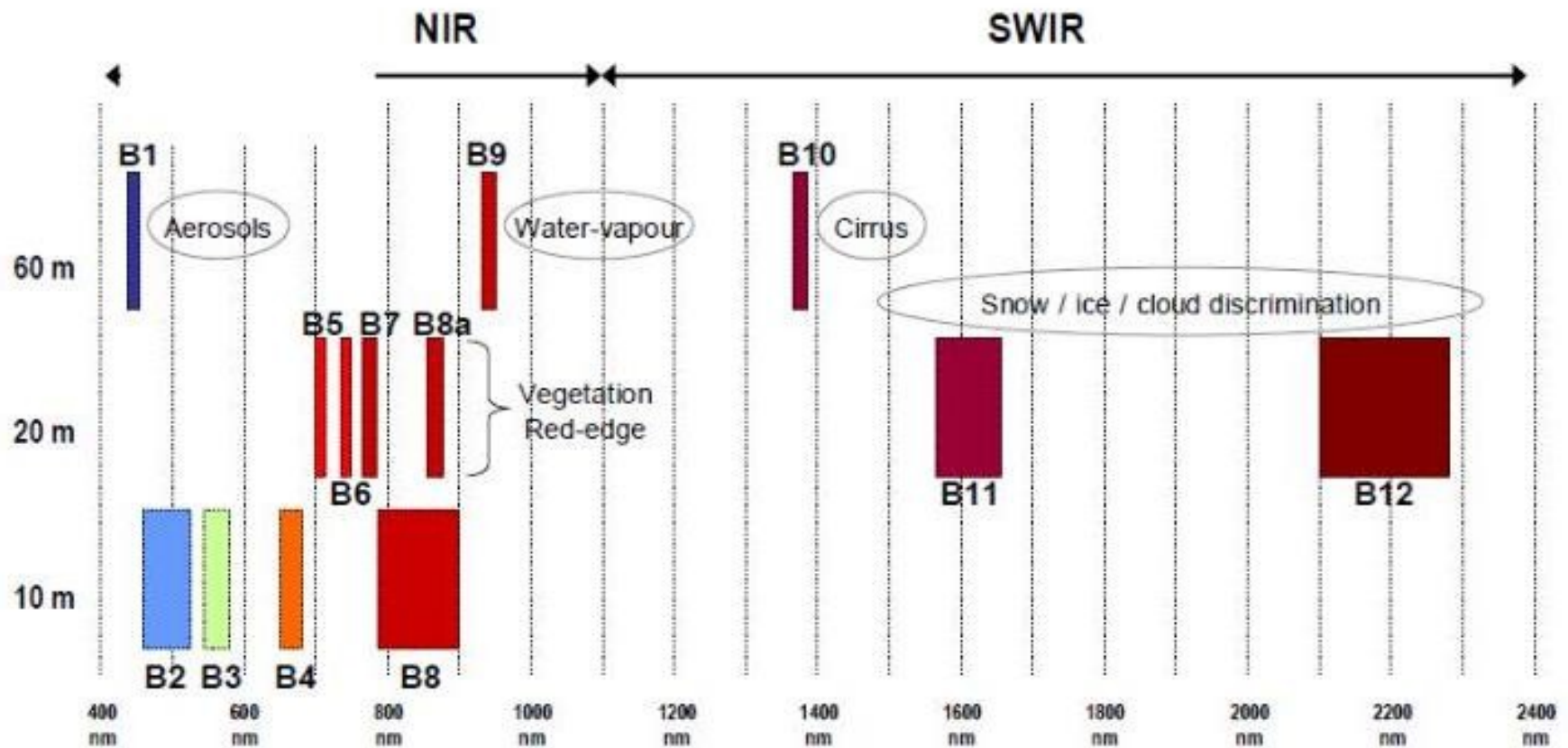
Figure 1: MSI Spectral-Bands versus Spatial Resolution
