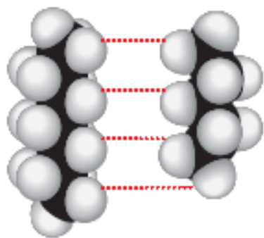
Eptano ( C_7H_{16} )
