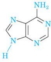
Adenina (A) DNA RNA
