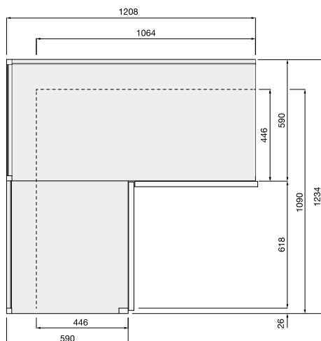
Con montante e fondali cristallo With upright and glass back panels
