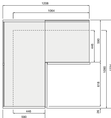
Con fianco e fondali legno With side and wooden back panels
