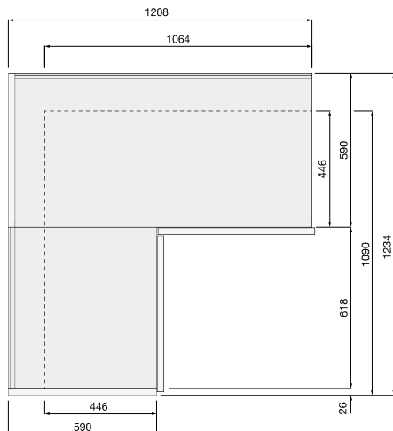
Con fianco e fondali legno With side and wooden back panels
