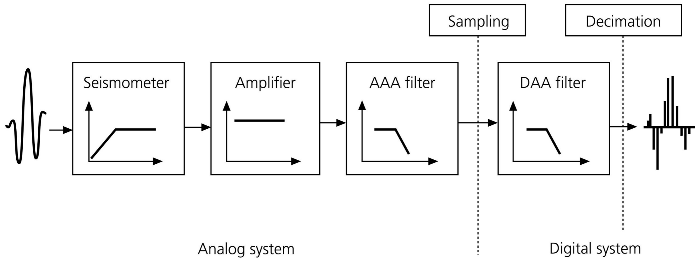
Figure 6.6-12: Diagram showing the analog-to-digital (ADC) process.
