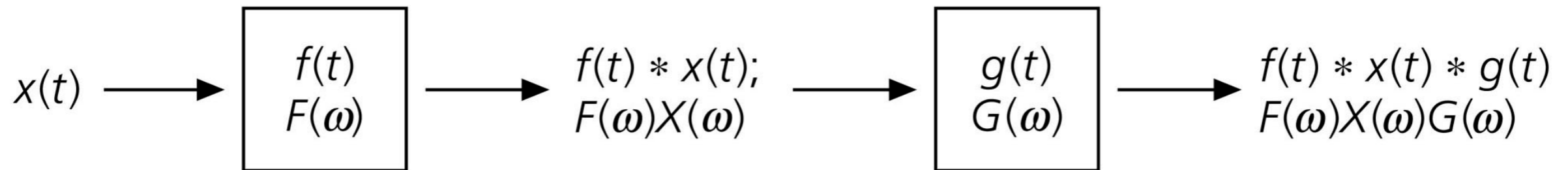
Figure 6.3-4: Two linear systems in succession.
