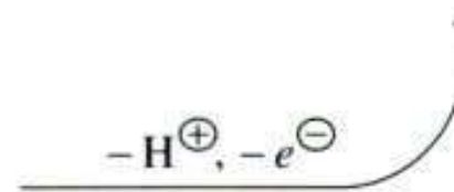
Flavoquinone (FMNH• or FADH•)
