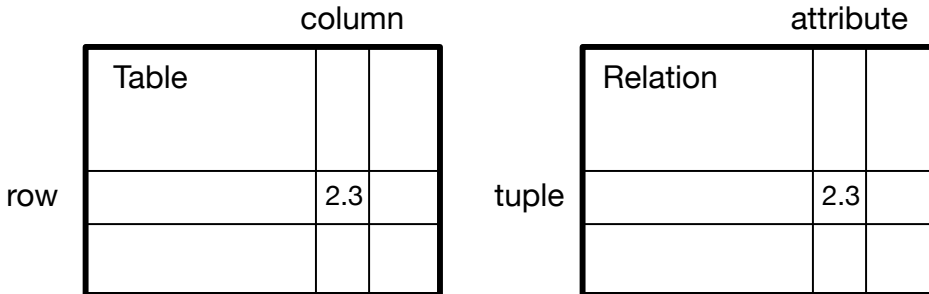
Figure 14.6: Relational Databases
