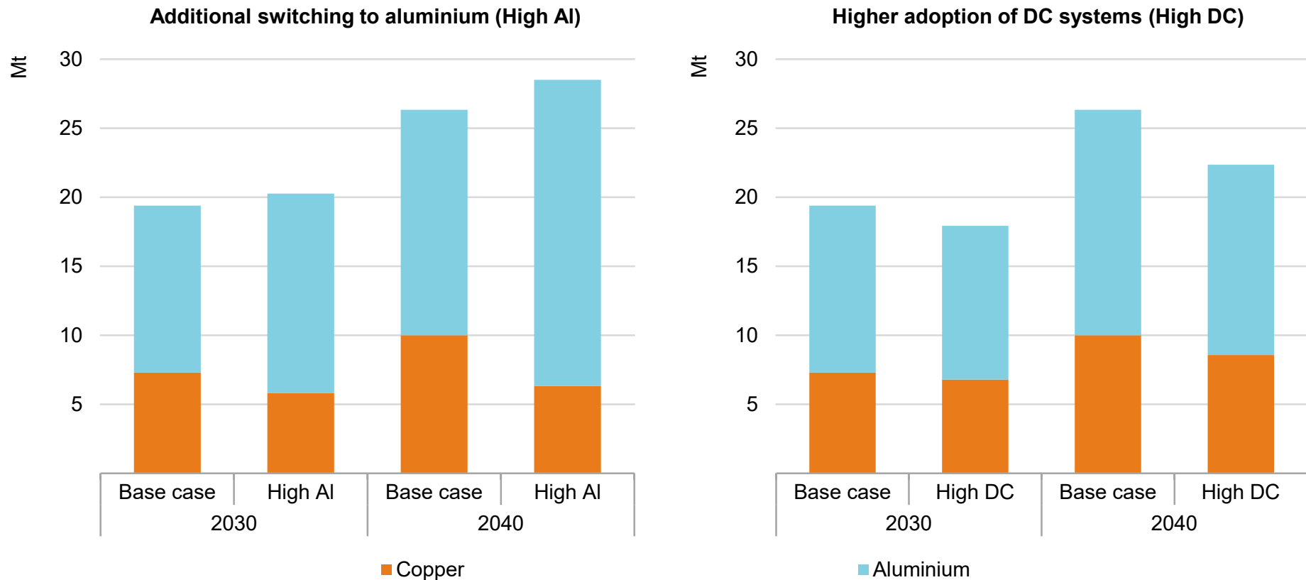
Copper and aluminium demand for electricity networks in the SDS under alternative cases
