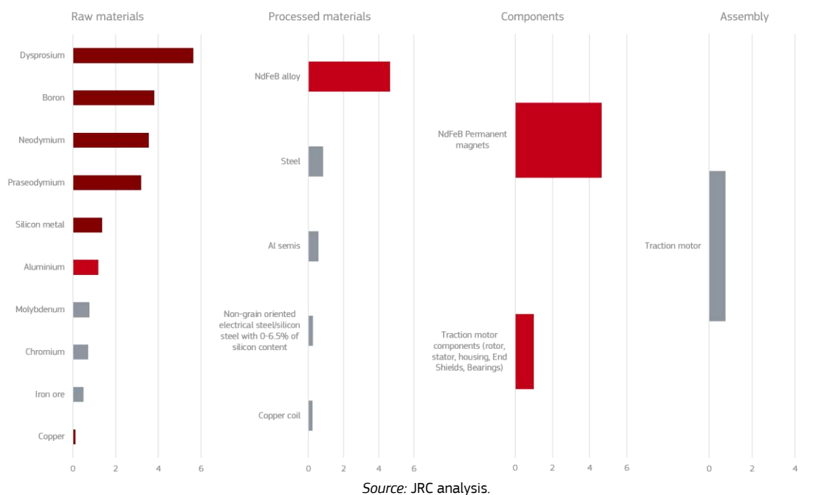
Figure 38. Detailed Supply Risk of all elements in the traction motors supply chain
