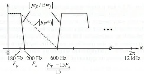
Figure 13.24: Decimation filter design based on the IFIR approach (frequency response plots not shown to scale).
