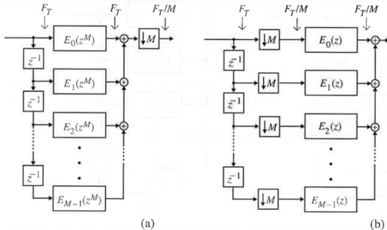
Figure 13.30: (a) Decimator implementation based on a Type I polyphase decomposition and (b) computationally more efficient realization.
