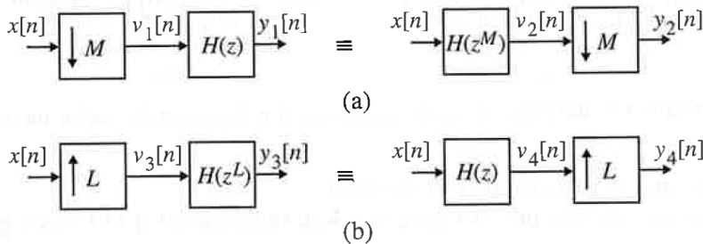
Figure 13.14: Cascade equivalences: (a) equivalence #1 and (b) equivalence #2.
