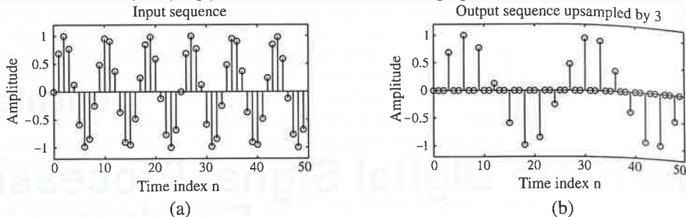
Figure 13.1: Illustration of the up-sampling process.
