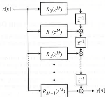
Figure 13.29: Realization of an FIR filter based on a Type II polyphase decomposition. Digital Signal and Image Processing
