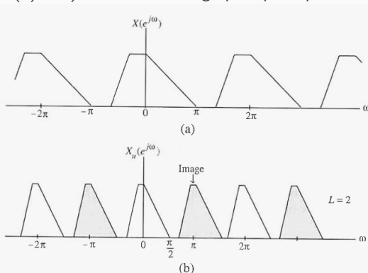
Figure 13.7: Effects of up-sampling in the frequency domain: (a) input spectrum and (b) output spectrum for L = 2 . Digital Signal and Image Processing
