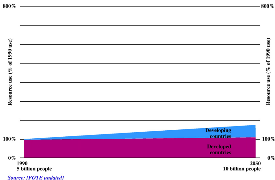
Fig. 5– Effects of predicted population growth on worldwide use of resources if current consumption and production patterns are maintained (1990=100%).
