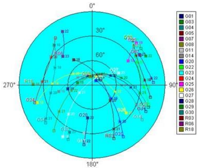
Sky Plot
