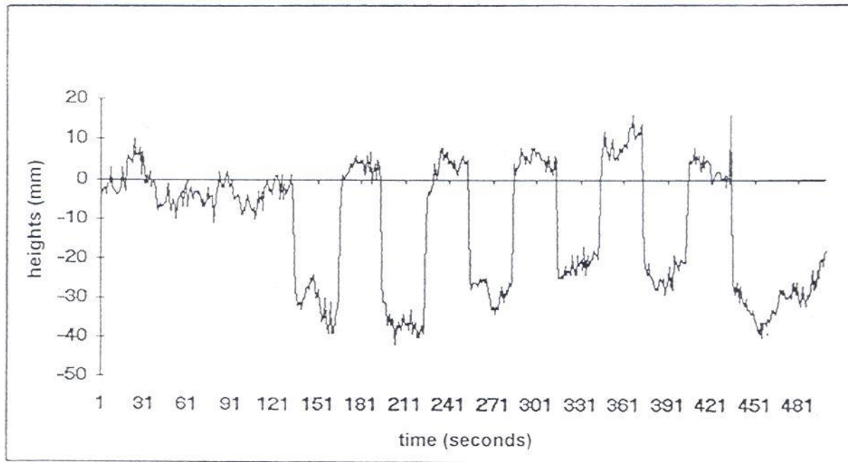
Fig. 2 - Real time display of the height variations moving the rove antenna of \pm 33 mm
