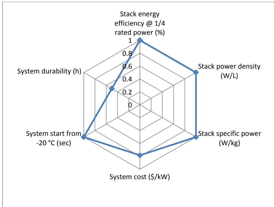
Figure 1. Fuel Cell Targets versus Status (The blue line indicates the status as a fraction of the targets)
