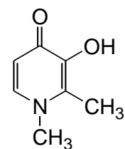
3,4-dihydroxypyridinone deferiprone
