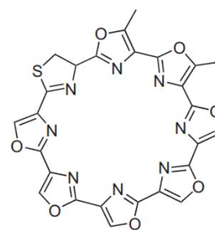
Telomestatin
