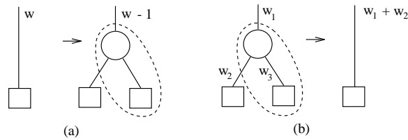
Fig. 1a,b. Update operations. (Only the involved nodes are depicted; the operations have symmetric variants. A circle denotes any node, a square denotes a leaf; a line without an associated weight denotes a black edge.) (a) Insertion: an internal node and a leaf are inserted. (b) Deletion: a leaf and an internal node are deleted.
