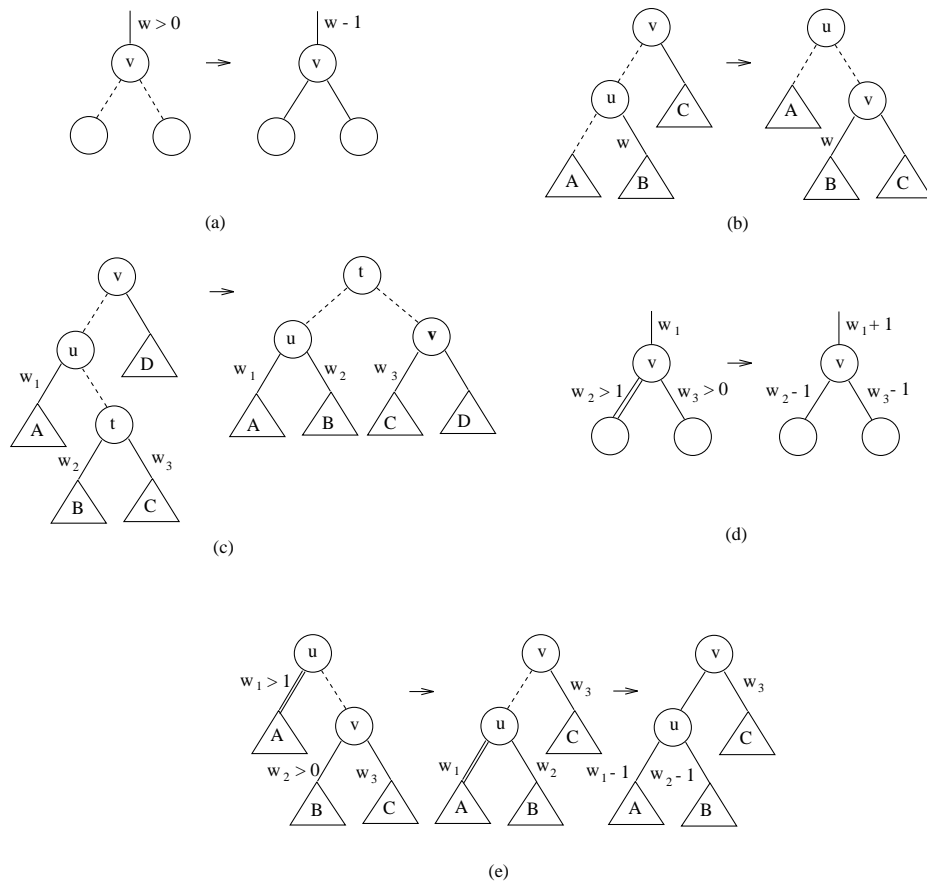
Fig. 2a–e. Rebalance operations. (All operations but (a) have symmetric variants. A broken line denotes a red edge, a double line denotes an overweighted edge; for other denotations see Fig. 1.) (a) Case 1 (the red child edges of the lowermost nodes are not shown): the weights are adjusted. (b) Case 2: a single rotation. (c) Case 3: a double rotation. (d) Case 4: the weights are adjusted. (e) Case 5: a single rotation is performed and the weights are adjusted.
