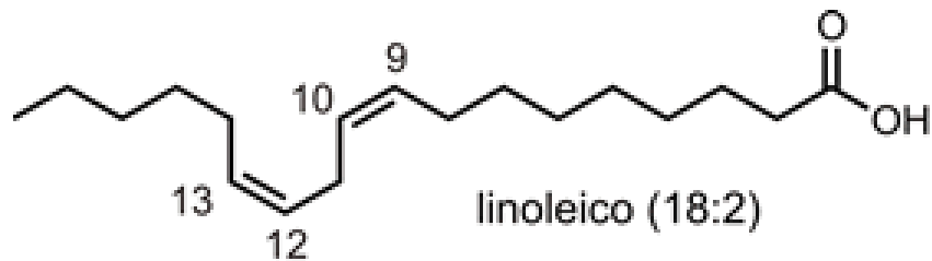
Acido linoleico 18:2 \Delta^{9,12} oppure 18:2 \omega 6
