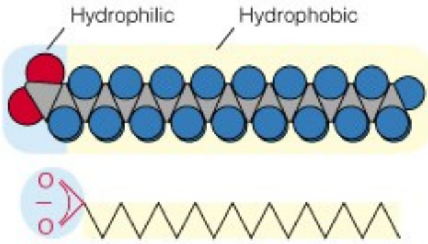
(a) Stearate ion
