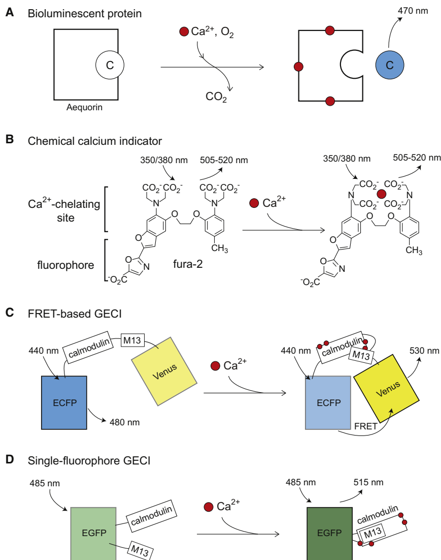
Figure 2. Calcium Indicators
