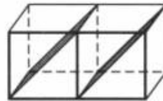
(0 \bar{1}\bar{1} )
