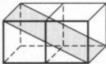
(012)
