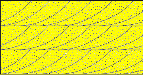
Cross-stratification
