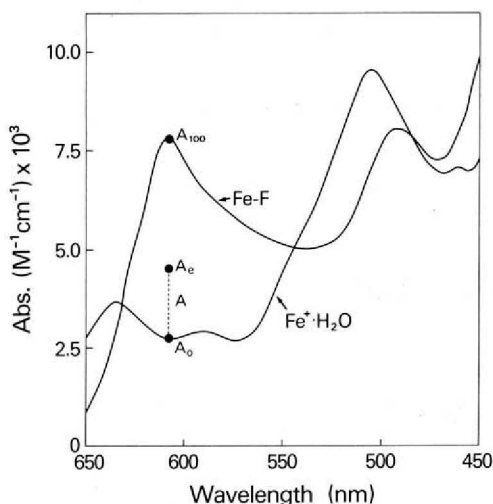
Figure 1. Main part of the absorption spectra, in the visible range, for ferri-myoglobin, \text{Fe}^+(\text{H}_2\text{O}) , and ferri-myoglobin-fluoride, \text{Fe-F} . Kinetic measurements were made at 608 nm where: A_0 = absorbance of ferri-myoglobin at start of reaction, A = absorbance (variable) during reaction, A_e = absorbance at point of equilibrium attained, and A_{100} = absorbance of fully formed ferri-myoglobin-fluoride product. Details are in the text.
