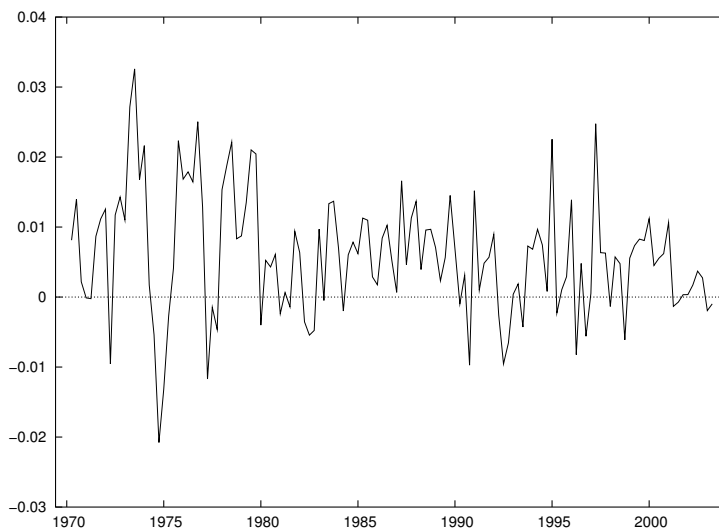
Figura 3.4: \Delta \log(\text{PIL})
