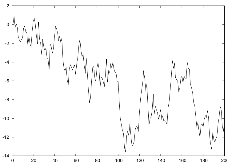
Figura 3.5: Random walk
