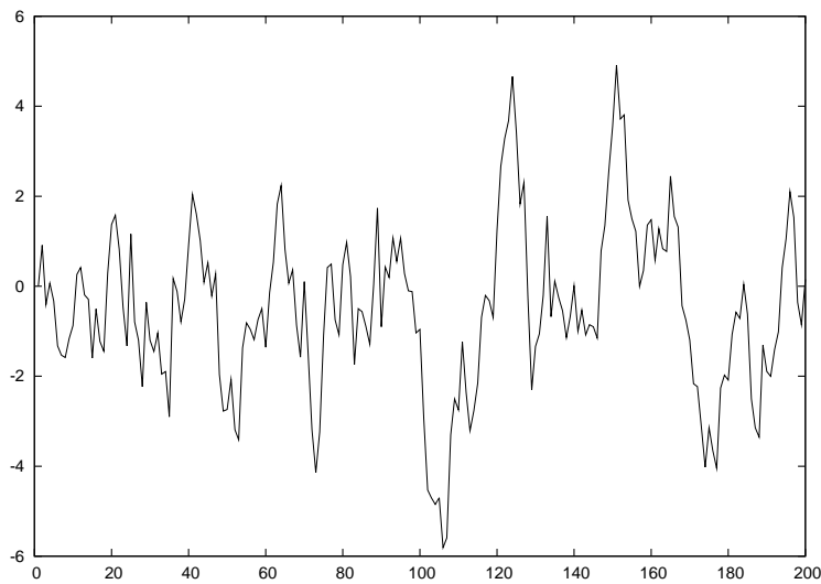
Figura 2.7: AR(1): \varphi = 0.9
