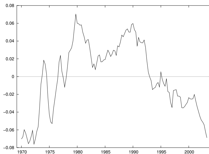
Figura 3.3: Residui
