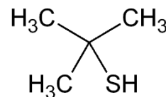
Tert-Butylmercaptan (added to methane)
