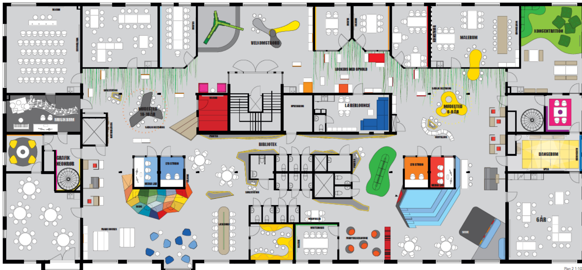
Vittra School, Brotorp, Stockholm. Planimetria generale.
