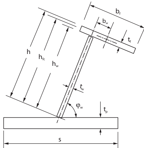
Figure 7 : Stiffener geometry (1/3/2008)
