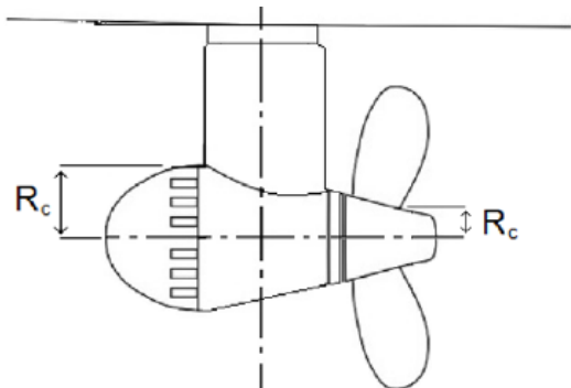
Figure 10 : Dimensions used for R_c (1/7/2020)
