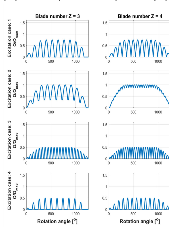
Figure 4 : The shape of the propeller ice torque excitation sequences for propellers with 3 and 4 blades (1/7/2020)
