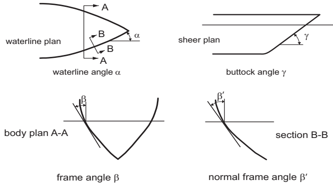
Figure 3 : Definition of hull angles (1/1/2012)
