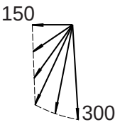
Figure 16 : Resultant permissible load on container corners
