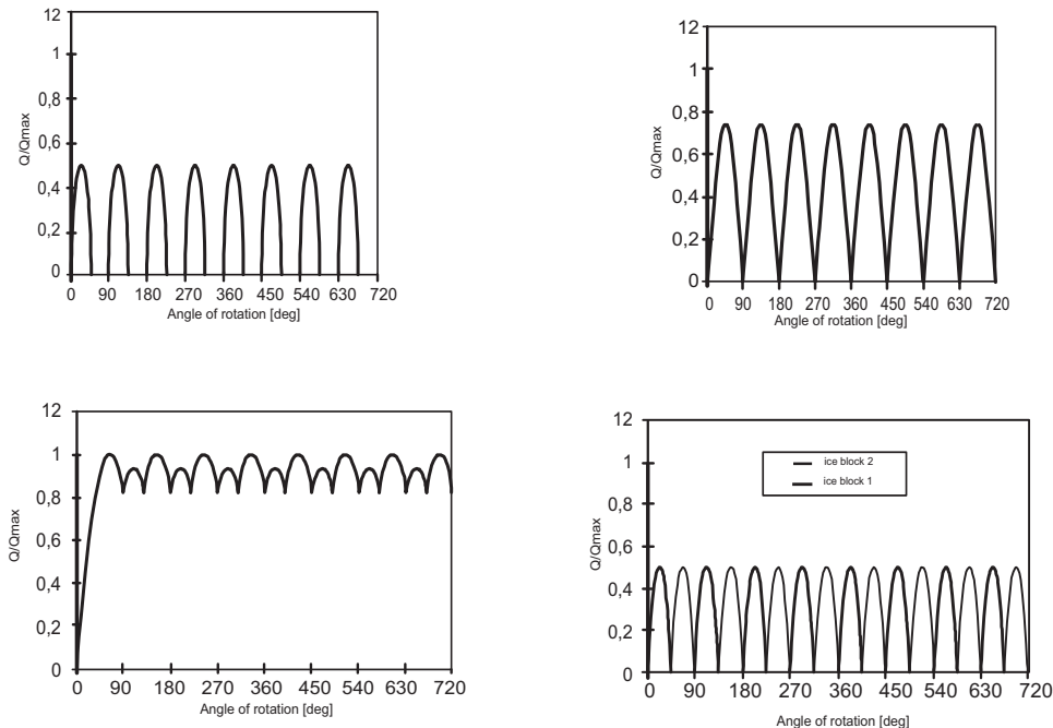
Figure 1 : Shape of the propeller ice torque excitation for 45, 90, 135 degrees single blade impact sequences and 45 degrees double blade impact sequence (two ice pieces) on a four-bladed propeller (1/3/2008)
