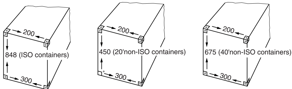
Figure 14 : Permissible transverse and vertical tensions on frames of 20' and 40' containers
