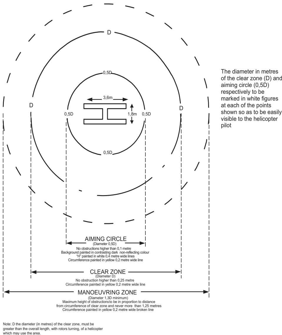
Figure 2 : Landing area without unobstructed access from ship's side (1/7/2010)
