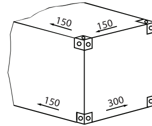
Figure 12 : Permissible transverse and longitudinal racking loads on frames of 20' and 40' containers (1/7/2015)
