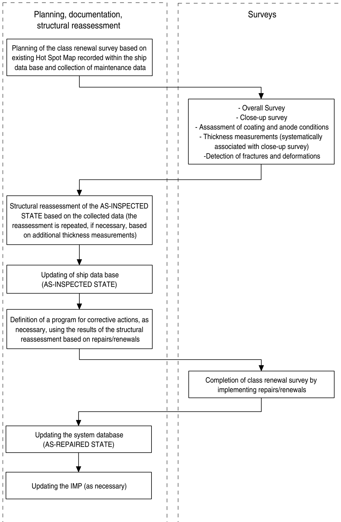
Figure 2 : Actions to be taken in connection with the Class Renewal Survey (1/11/2022)
