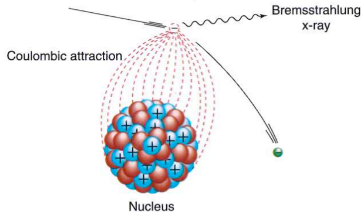
■ FIGURE 3-4 Radiative energy loss via bremsstrahlung (braking radiation).
