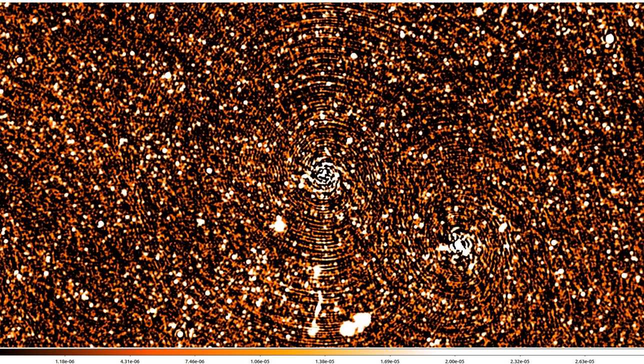
MeerKAT Observations on the Spiderweb (PI Pannella)
